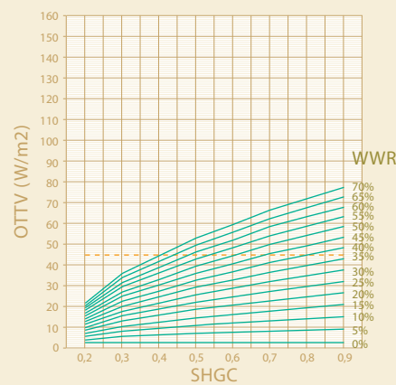
WWR Dinding Barat (270°)
